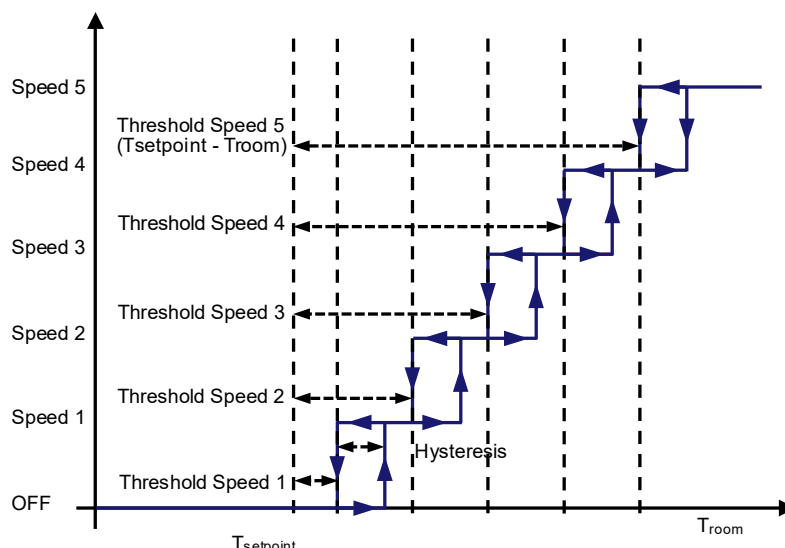
Fig. 64: Fan Controller 2-Points Control Cycle for Cooling
