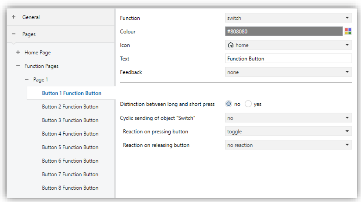
Fig. 12: Function Page - Button X Configuration Page
