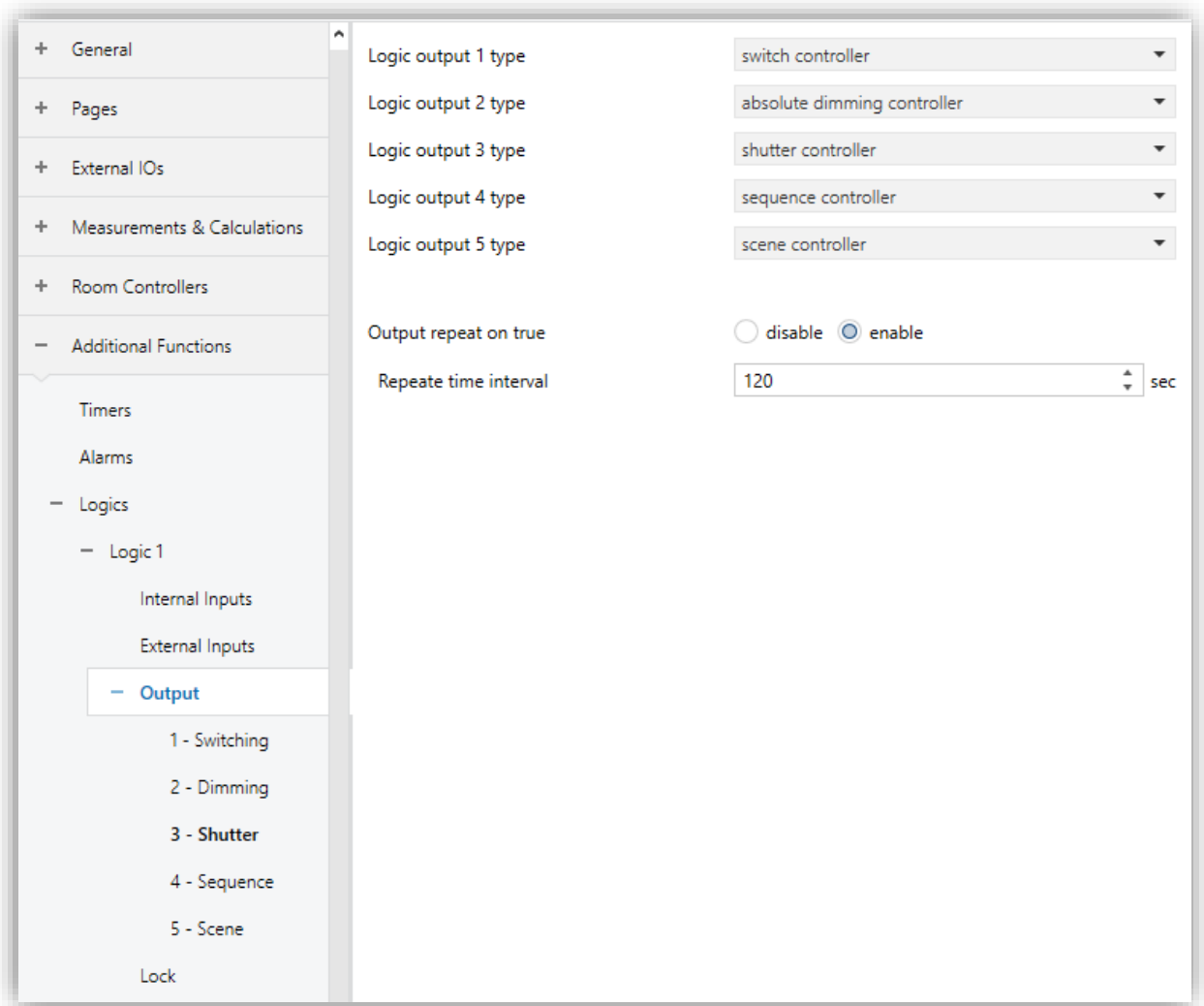
Fig. 80: Logics – Output 1-5 Configuration Page
