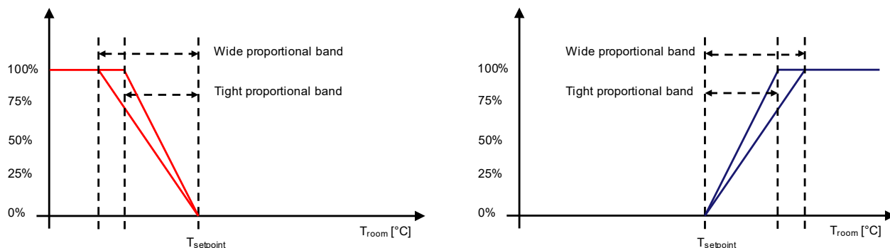
Fig. 42: Continuous PI Control Proportional Band Widths
