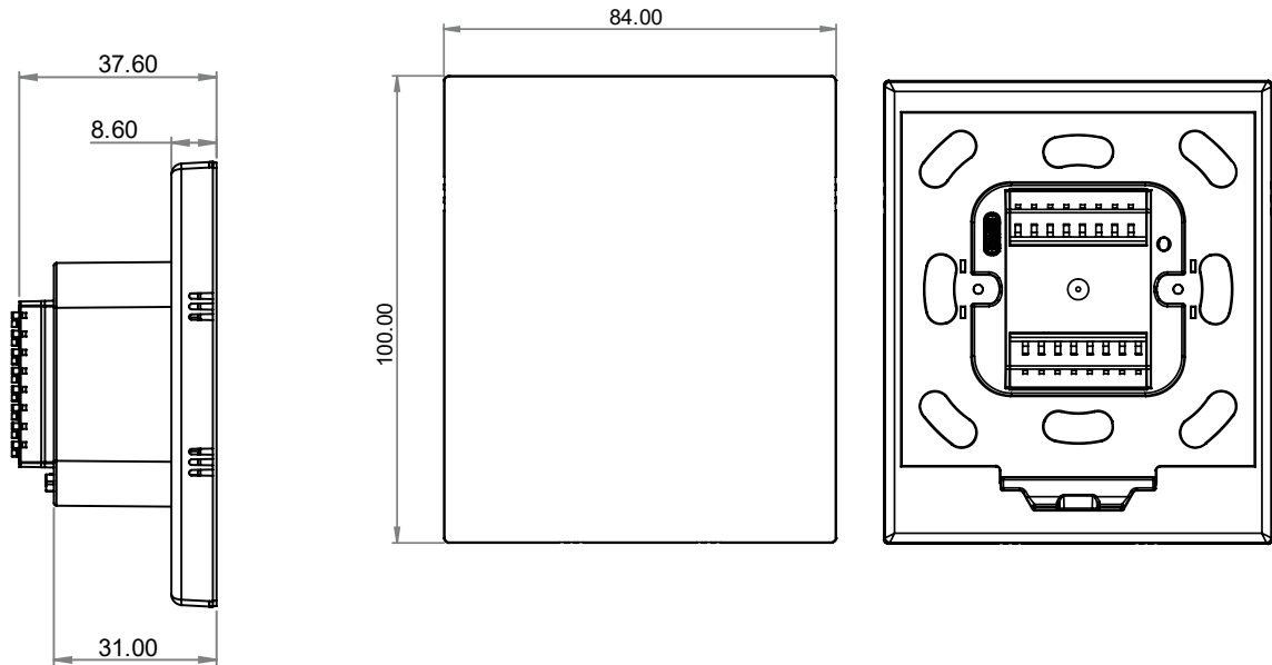
Fig. 1: Dimensions of the iX4
