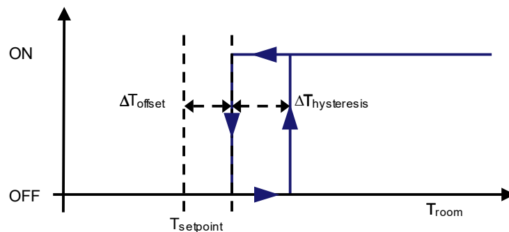
Fig. 56: 2 – Points Hysteresis Cycle for Additional Cooling Control
