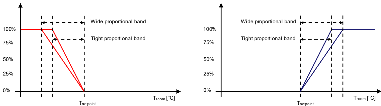
Fig. 66: Fan Controller Proportional Control
