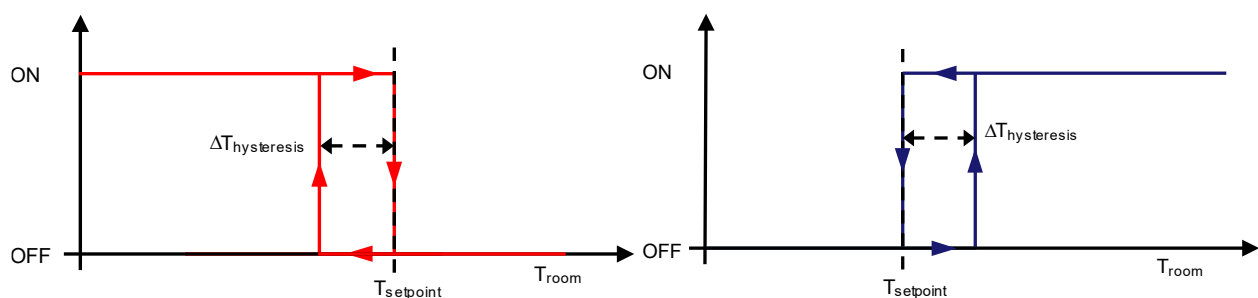
Fig. 41: 2 – Points Control Hysteresis Cycle
