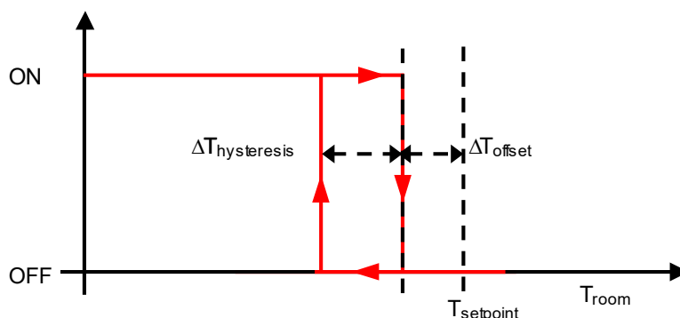
Fig. 50: 2 - Points Hysteresis Cycle for Additional Heating Control
