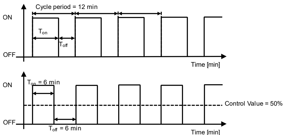
Fig. 43: PWM Control Sampling
