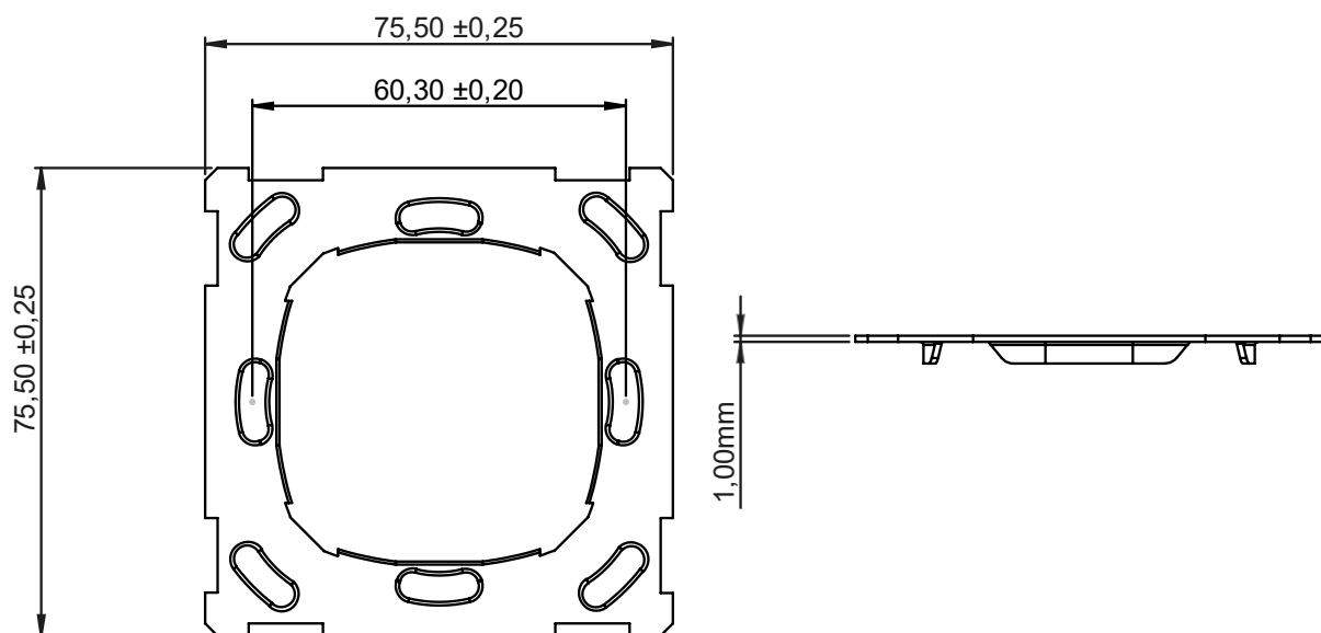
Fig. 2: Dimensions of the iX4 Mounting Plate
