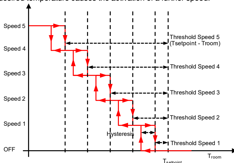
Fig. 63: Fan Controller 2-Points Control Cycle for Heating
