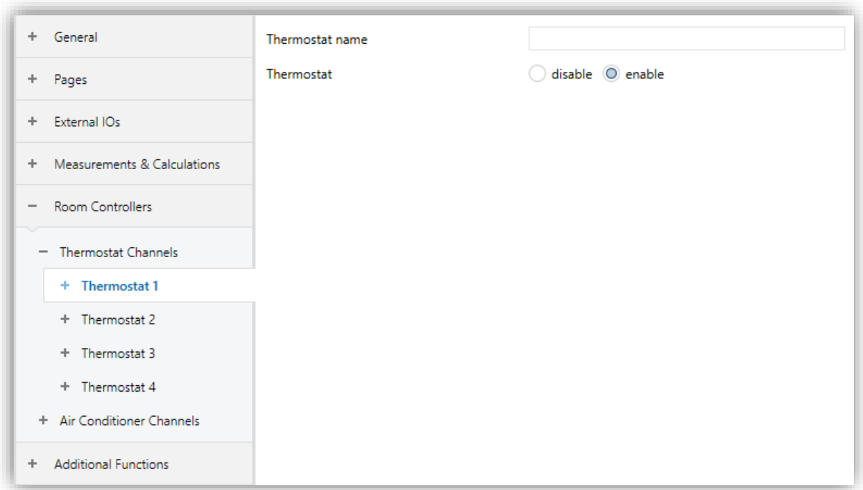
Fig. 44: Room Controller Thermostat Configuration Page
