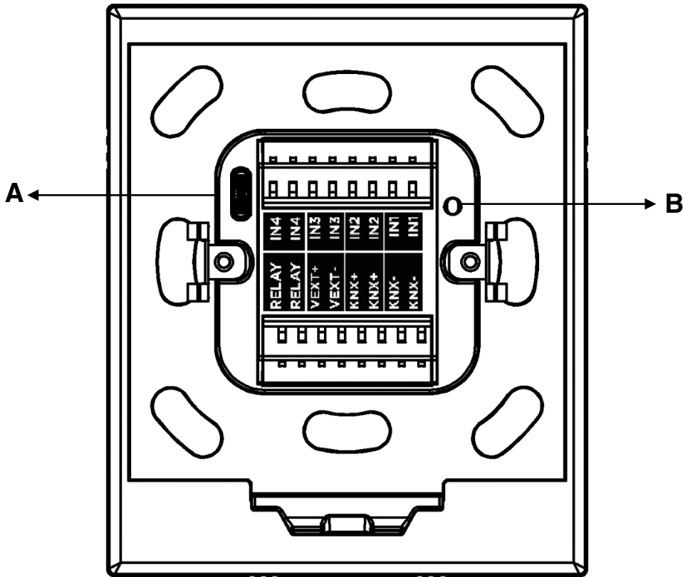
Fig. 3: Connection to KNX and Programming Button
