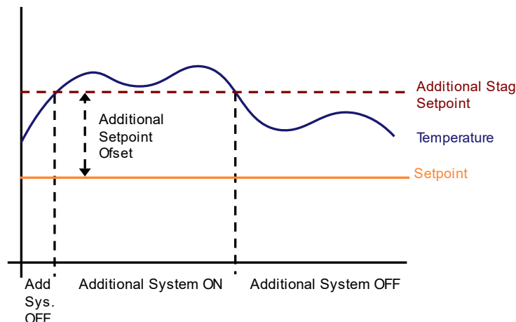
Fig. 57: PI Continuous Graph for Additional Cooling Control
