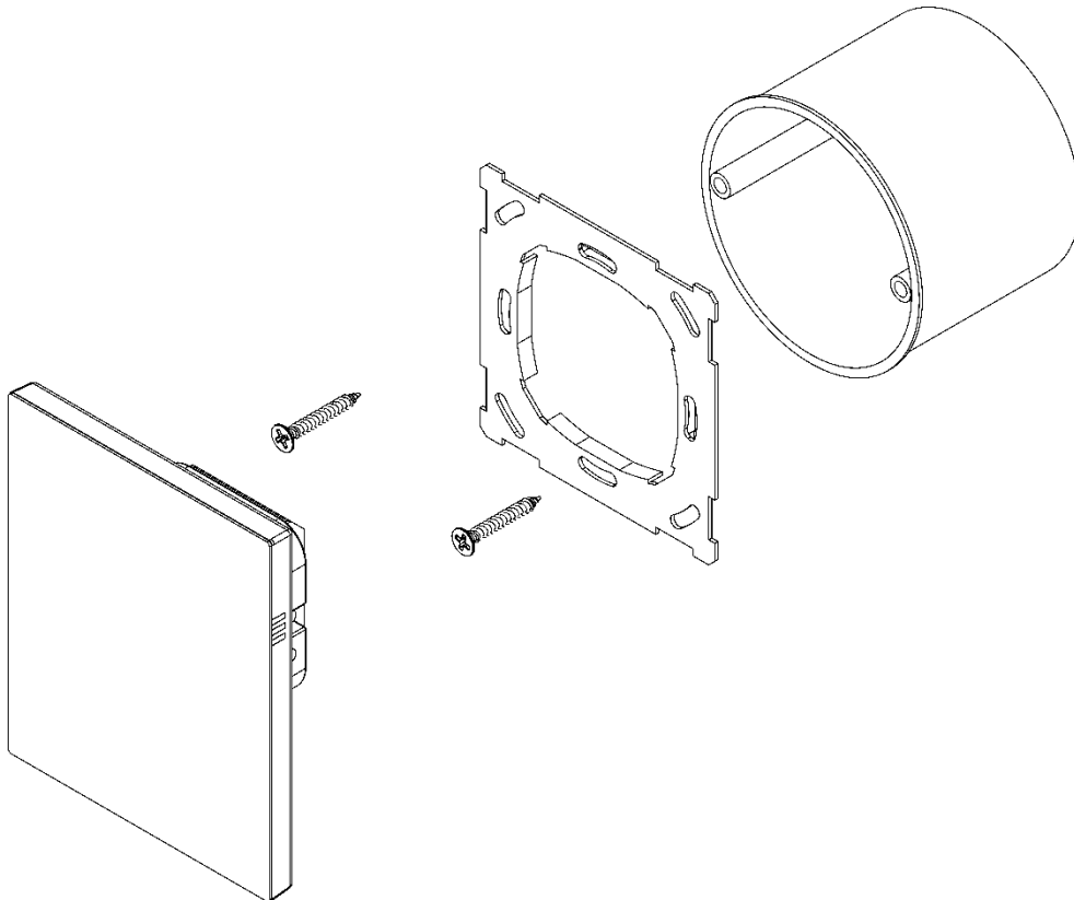
Fig. 4: Mounting the to Flush Mounting Box
