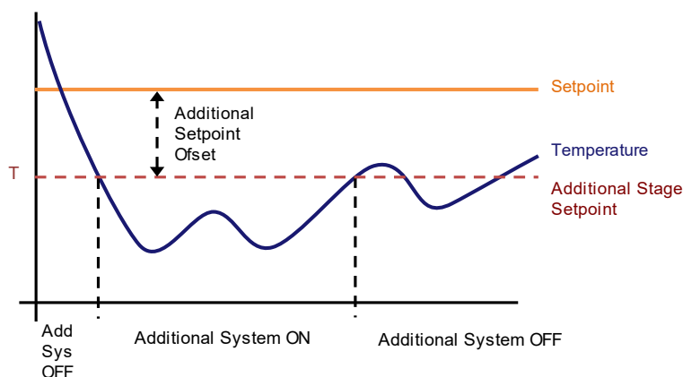
Fig. 51: PI Continuous Graph for Additional Heating Control
